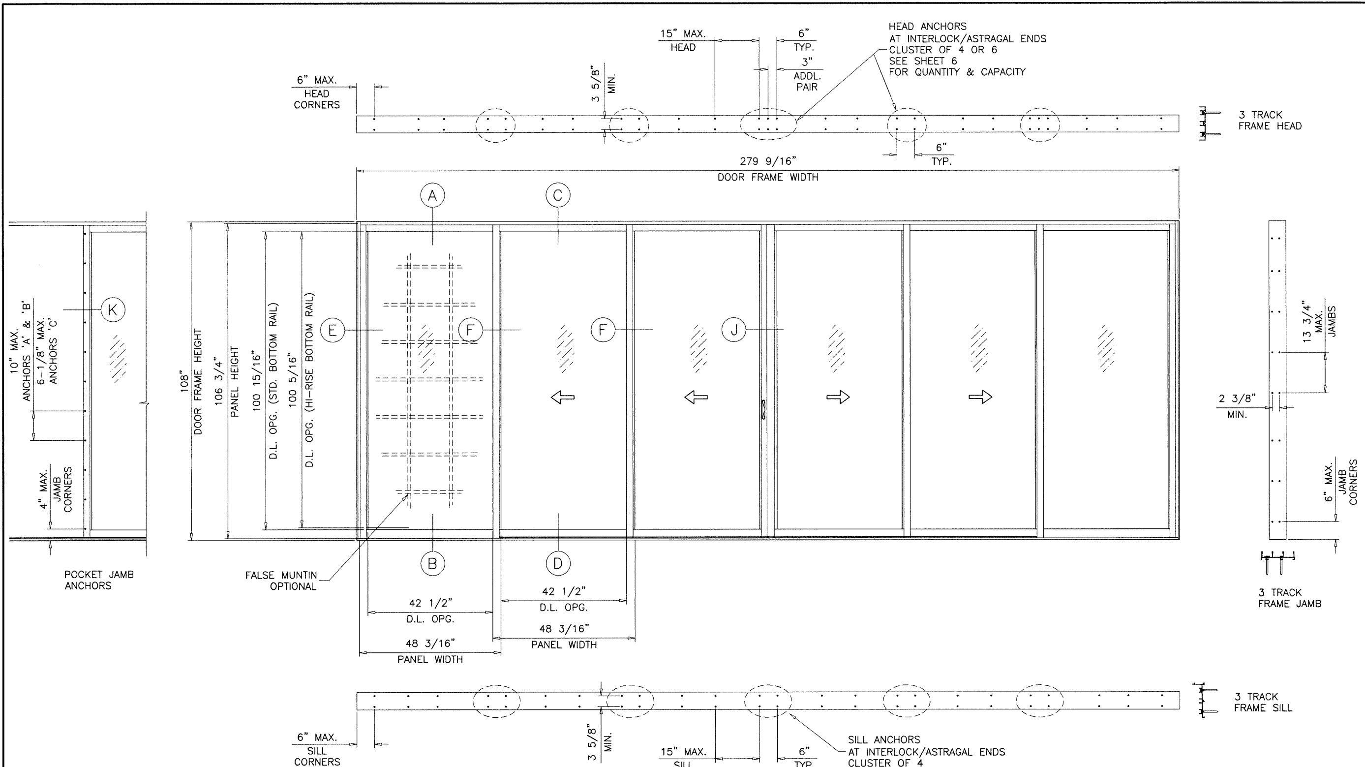
TYPICAL ELEVATION OXX-XXO
