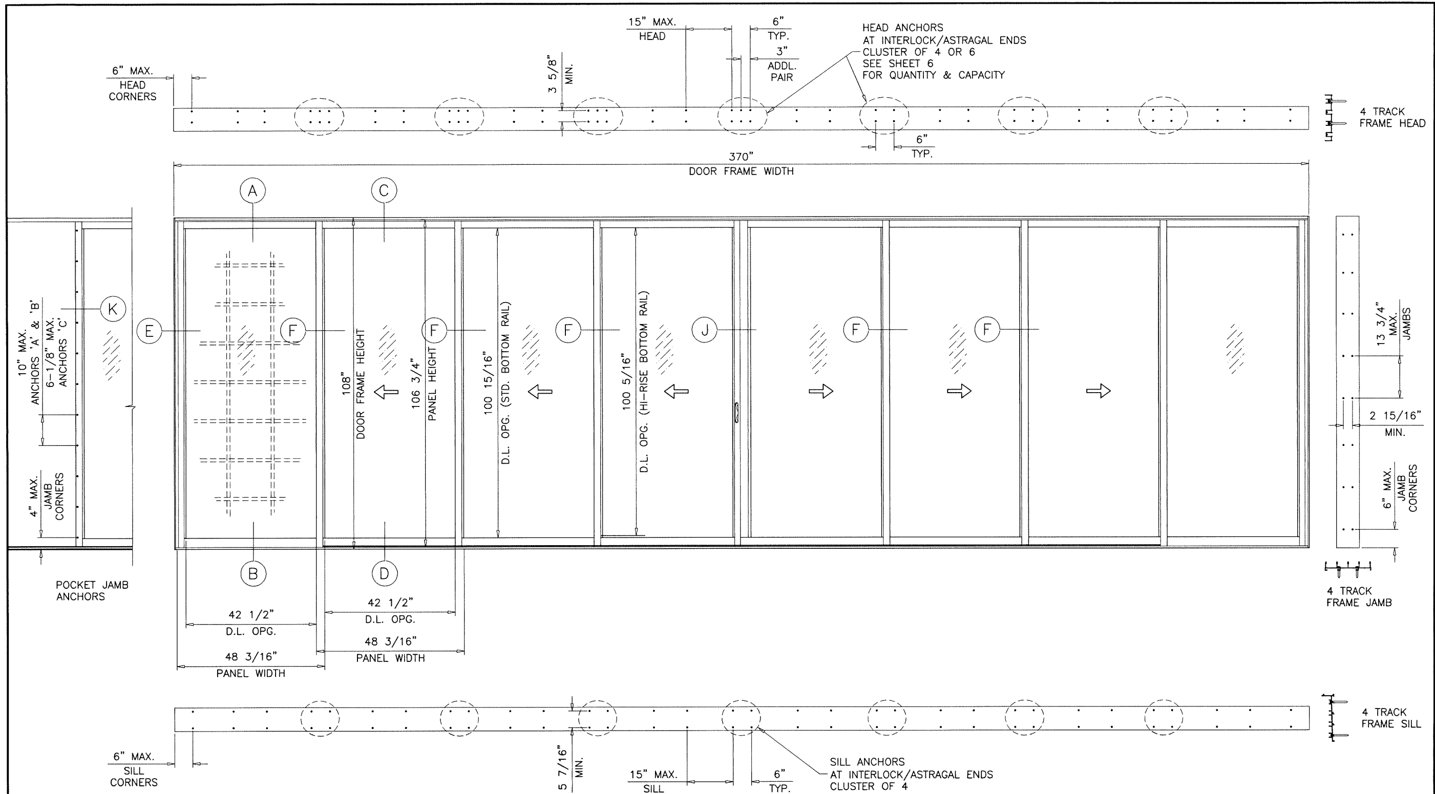
TYPICAL ELEVATION OXXX-XXXO
