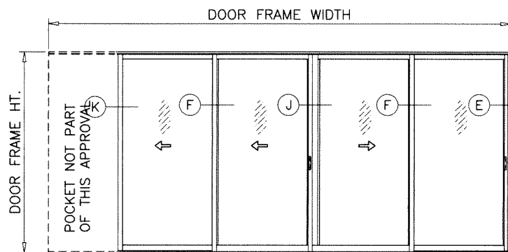
PXX-XO (SHOWN) OX-XXP
